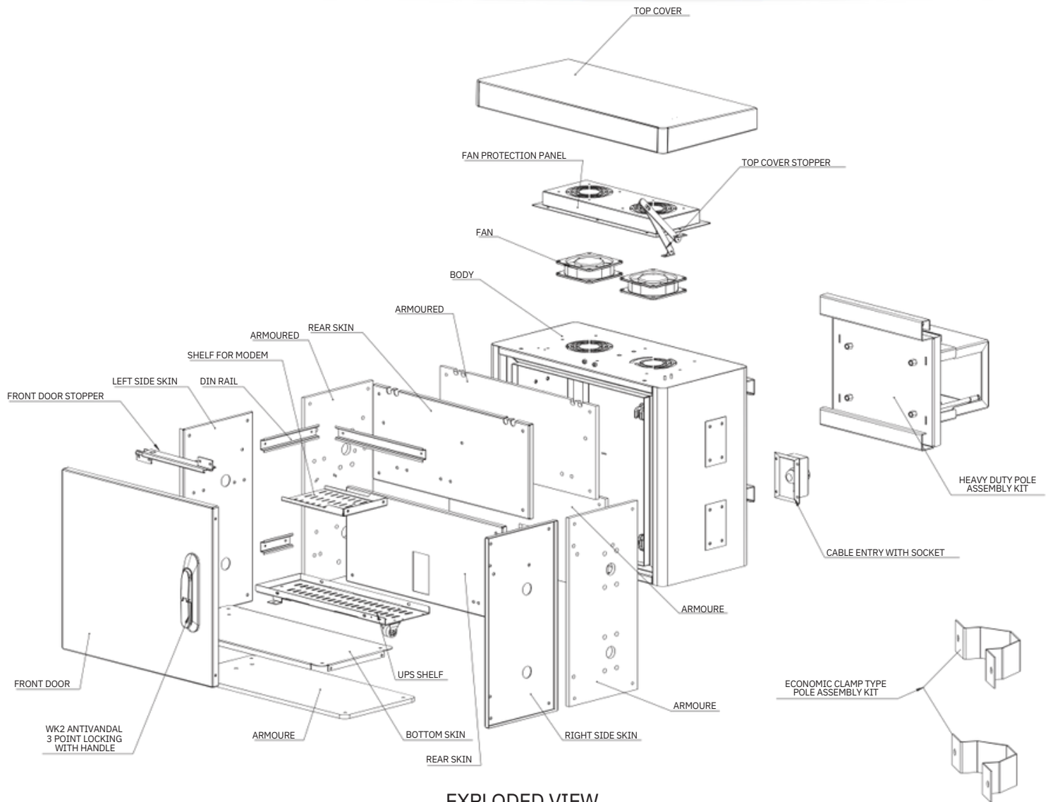
EXPLODED VIEW
