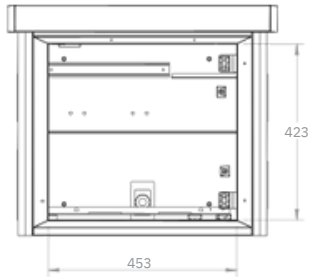
WITHOUT FRONT DOOR VIEW
