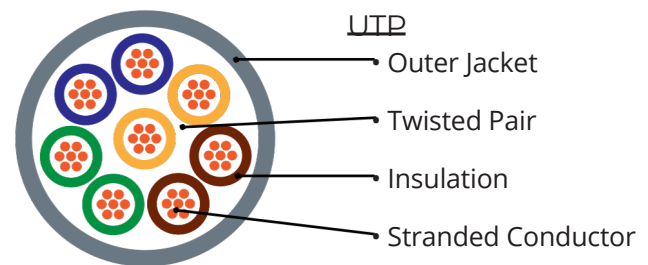
Figure 2: Cable Structure
