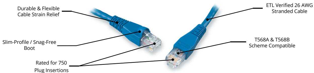
Figure 3: Category 6 -115 Series Detail
